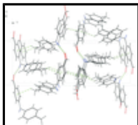
Fig. 2. The crystal packing of the title compound. Intermolecular hydrogen bonds and C—H... \pi contacts are shown as dashed lines.
